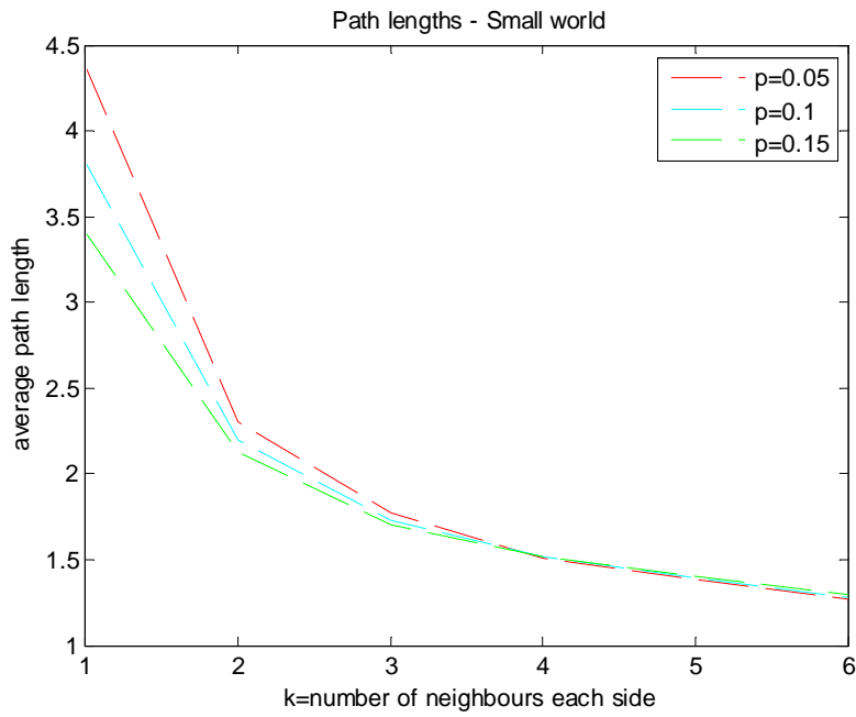
Figure 3 Average path length of small world network with 17 vertices, average over 500 separate realisations; rewiring replaces immediate neighbour connections; p is the probability of re-wiring, k is the number of immediate neighbours
