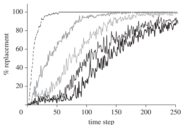
Figure 1. The effect of the simple memory parameter on replacement rate under the simple neutral model, with N = 1000 , and \mu = 10\% . Here we consider an original vocabulary of 100 popular words, and how those words are replaced over time under the model (note that an ‘S’ curve does not follow from the simpler version of the model, where m = 1 ). Dashed line, m = 1 ; thick grey line, m = 5 ; thin grey line, m = 10 ; thin black line, m = 15 ; thick black line, m = 20 .
